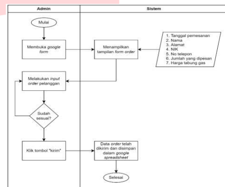
Gambar II. 9 Activity Diagram
