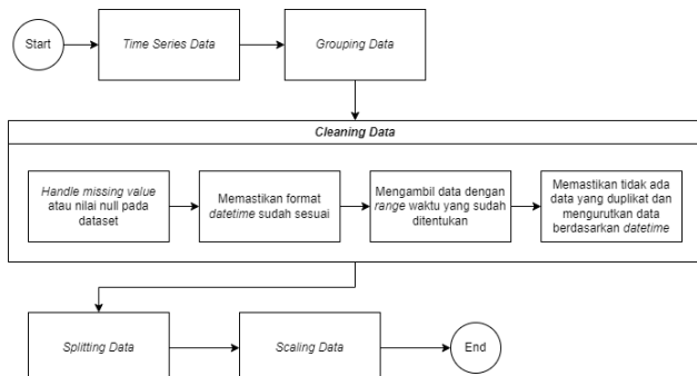
GAMBAR III.3 Rancangan Data Preparation
