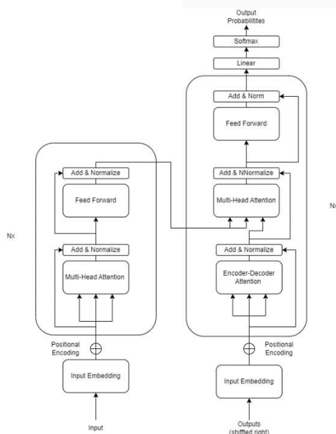
FIG 1. Transformer Architecture
