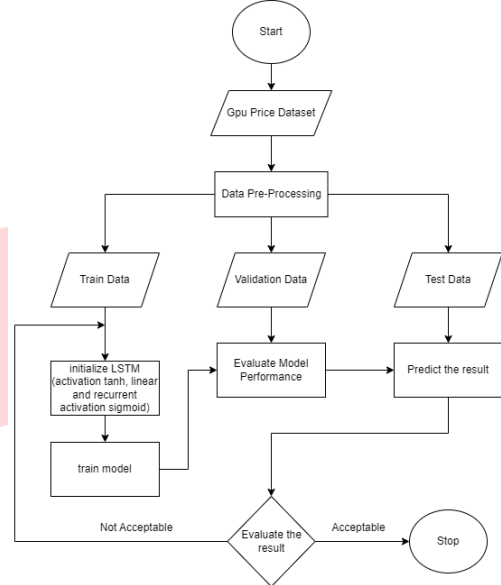
FIG 8. LSTM flowchart
