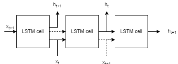
FIG 6. LSTM architecture
