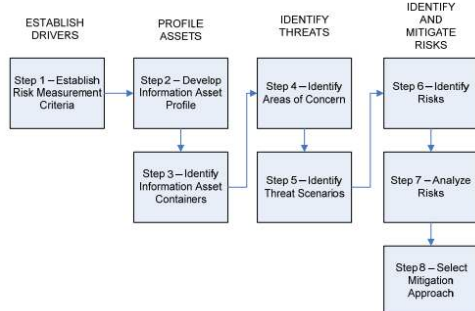
GAMBAR 1 OCTAVE Allegro Roadmap
