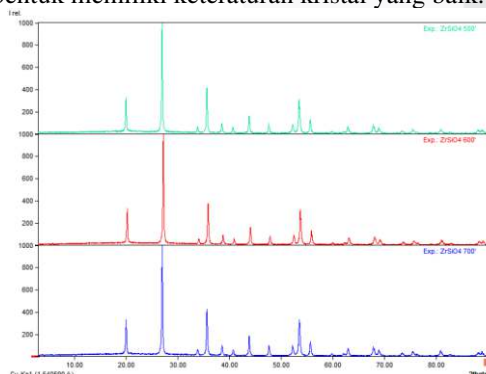
GAMBAR 2. Grafik X-Ray Diffraction (XRD)
