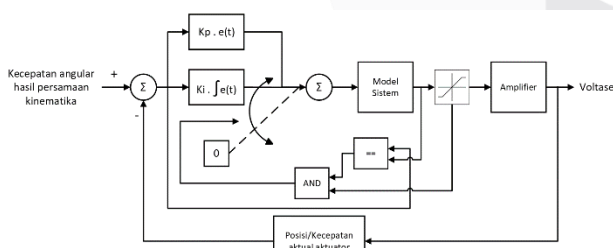
GAMBAR 10. Diagram block Solusi Metode Kendali PID (C)
