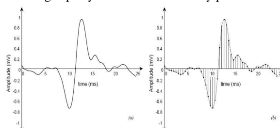
Gambar 2. Proses sampling . (a) sinyal analog (b) hasil sampling
