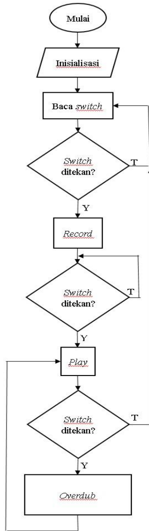
Gambar 9. Diagram alir footswitch
