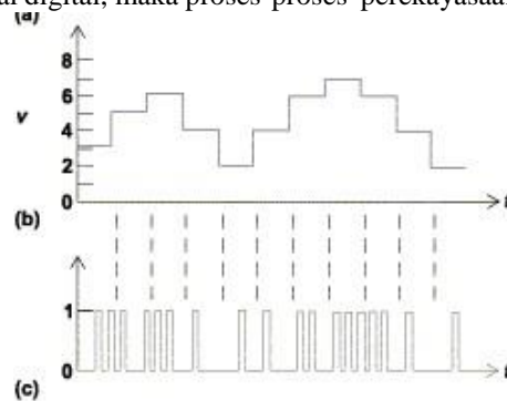
Gambar 4. Proses encoding .
