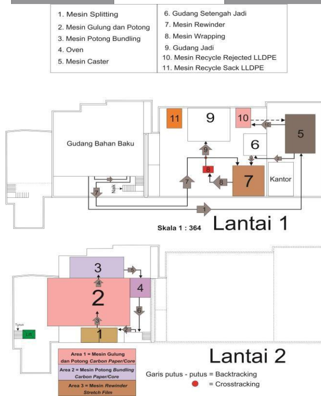
Gambar 2.4 Layout Usulan
