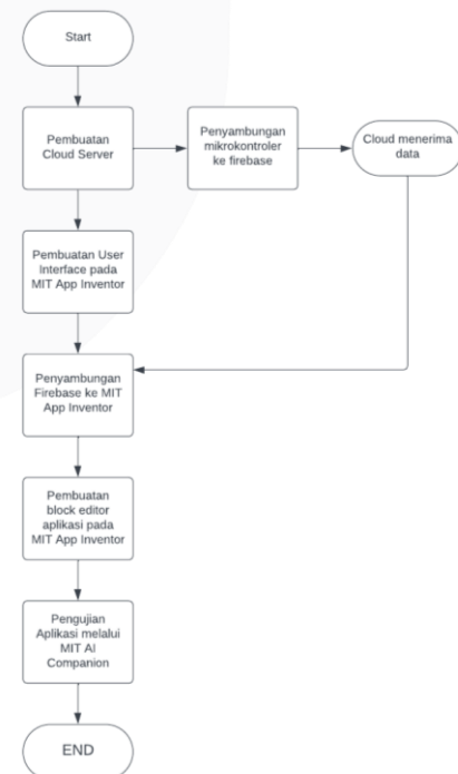
GAMBAR 5 (Flowchart Sistem)
