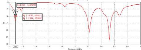
Gambar 18 Optimasi Return Loss ADS-B
