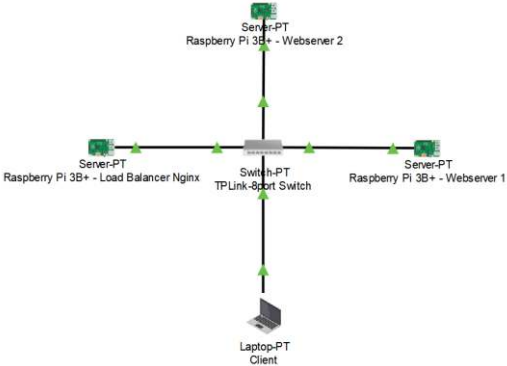
FIGURE 3.1. System Topology
