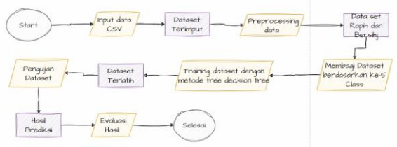
GAMBAR 4 (Flow Metode Decision Tree )
