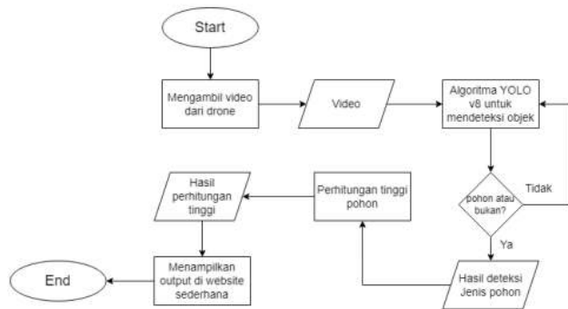
GAMBAR 5 flowchart system
