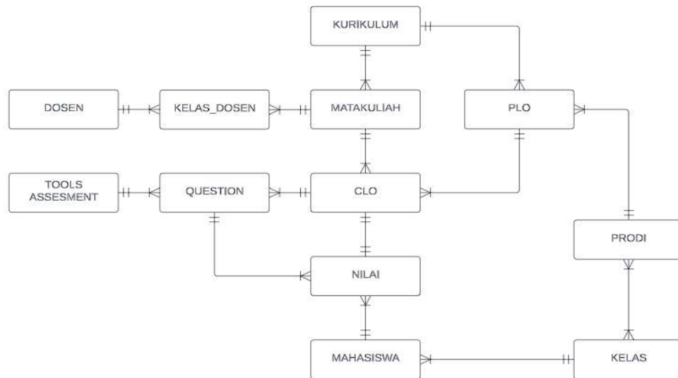
Gambar 3. 3 Diagram sistem
