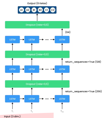
GAMBAR 10. Arsitektur RNN-LSTM matriks Fluency
