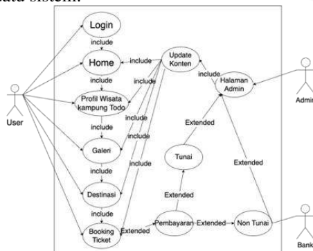
GAMBAR 2 (Metode Use Case Diagram )
