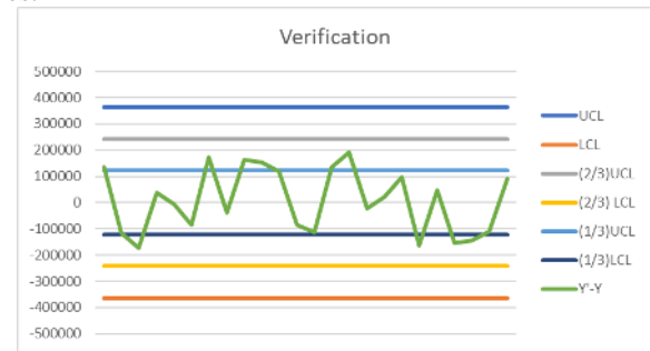
FIGURE 5 Out-of-control Verification
