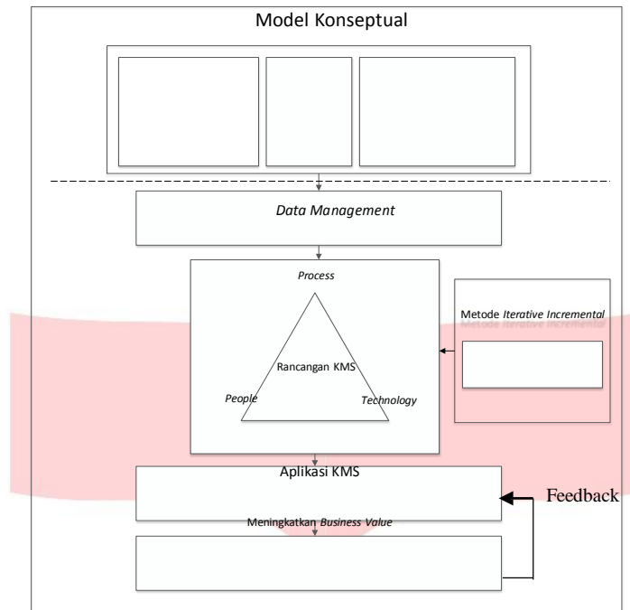
Gambar 3.1 Model Konseptual
