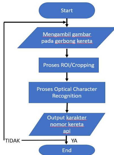
Gambar 4. Flowchart
