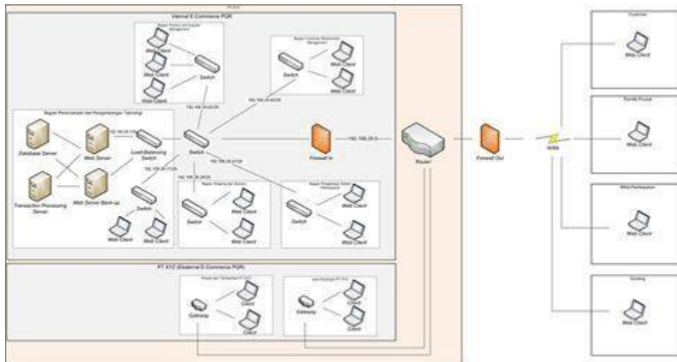
Gambar 10. Environment and Locations Diagram PQR (Target)
