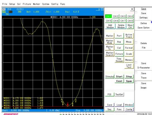
Gambar 4.1 (a) Hasil pengukuran VSWR di Network Analyzer
