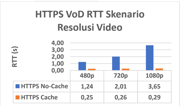
GAMBAR 8: Grafik VoD RTT Skenario Resolusi Video
