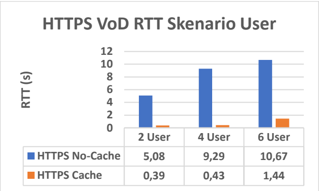
GAMBAR 5: Grafik VoD RTT Skenario User
