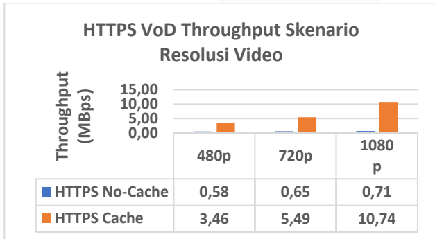
GAMBAR 6: Grafik HTTPS VoD Throughput Skenario Resolusi Video
