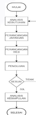
GAMBAR 1. Flowchart Penelitian
