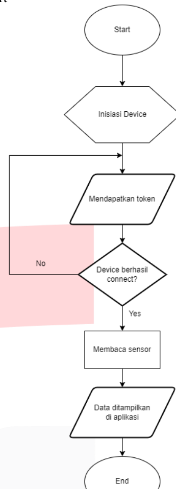
GAMBAR 2 Flowchart
