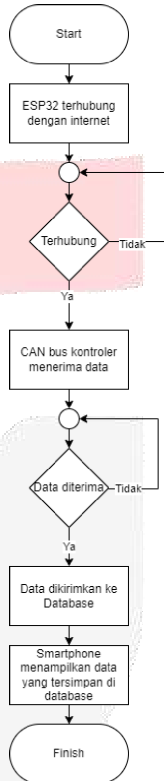
GAMBAR 3.3 Flowchart sistem
