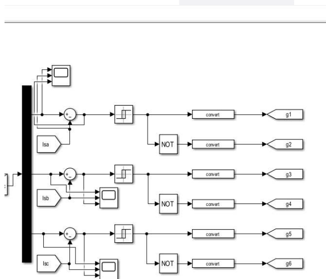
GAMBAR 3 Inverter
