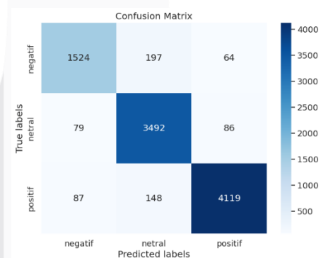
GAMBAR II-3 Confusion matrix Prabowo
