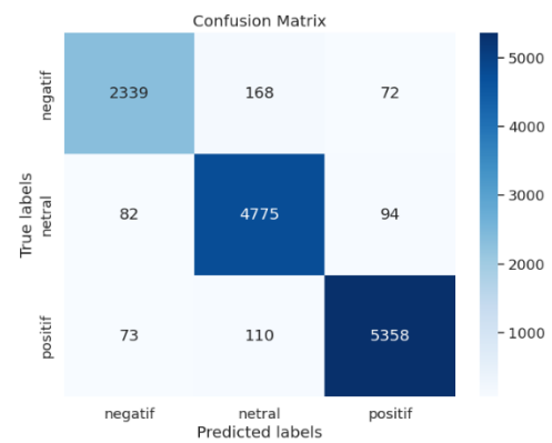
GAMBAR II-2 Confusion matrix anies
