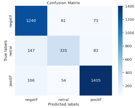
GAMBAR II-4 Confusion matrix ganjar
