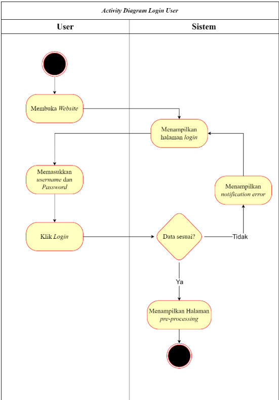
GAMBAR III.7 (Activity Diagram)
