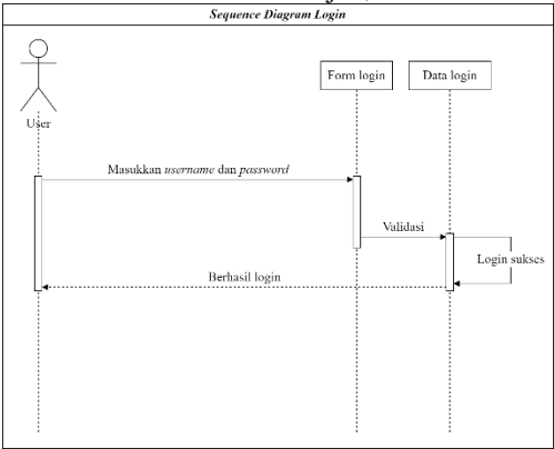
GAMBAR III.8 (Sequence Diagram)
