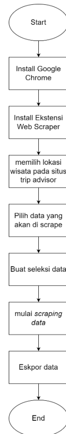
Gambar III.4 (Proses Web Scraping )
