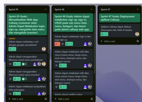
GAMBAR 6. Sprint Planning
