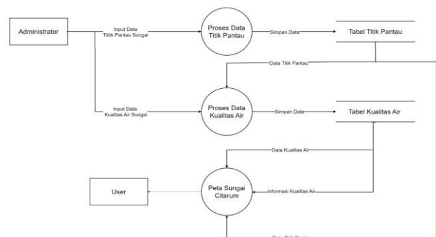
GAMBAR 3.2 Data Flow Diagram Level 1
