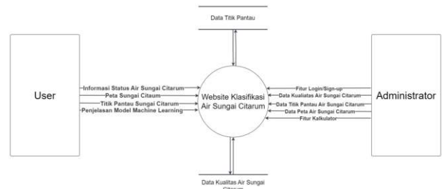
GAMBAR 3.1 Data Flow Diagram Level 0
