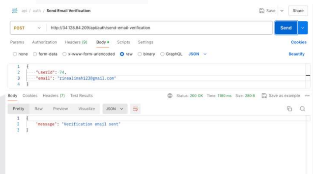
GAMBAR 3 Hasil Test Endpoint API Email Verification
