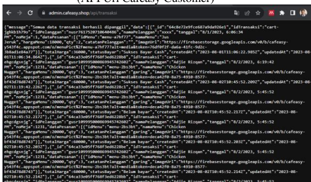
GAMBAR 4 (API Url Cafeasy Admin)
