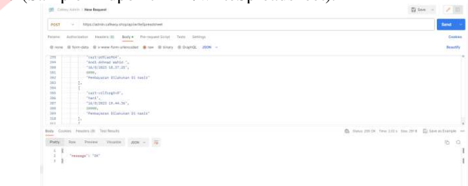
GAMBAR 7 (Sample Endpoint API /writeSpreadsheet)
