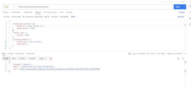
GAMBAR 9 (Akses Endpoint API Midtrans Payment)
