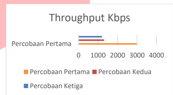
GAMBAR 8 Throughput
