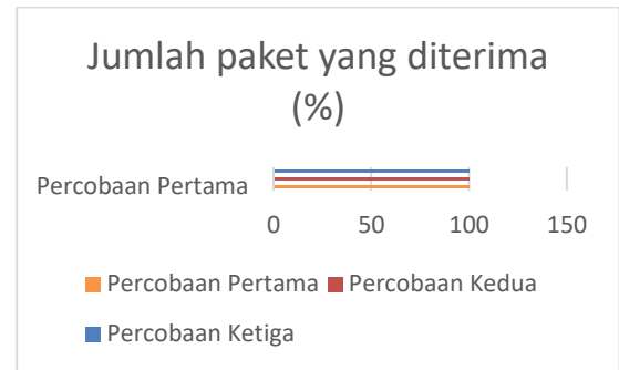
GAMBAR 7 Packet Loss
