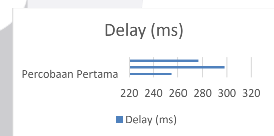
GAMBAR 9 Delay
