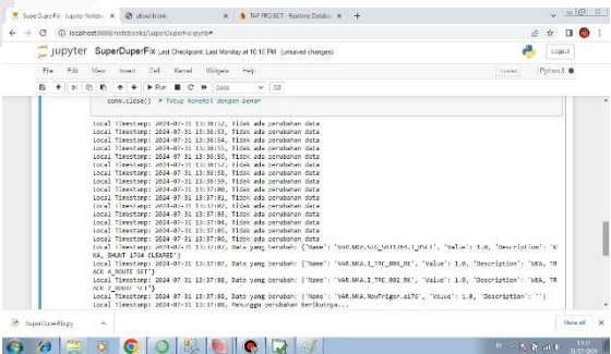
GAMBAR 4.3 Output Python
