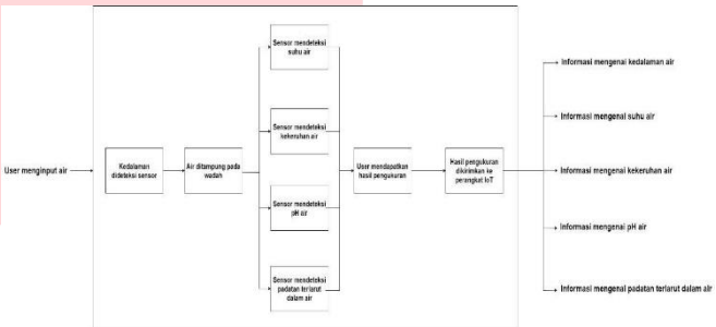
GAMBAR 5 Diagram Blok Level 1 Sistem monitoring kualitas air
