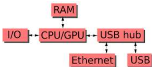
GAMBAR 2. 2 Diagram blok Raspberry Pi 4
