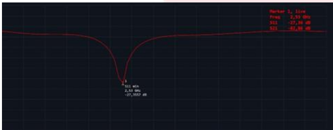
GAMBAR 4.5 RETURN LOSS REALISASI
