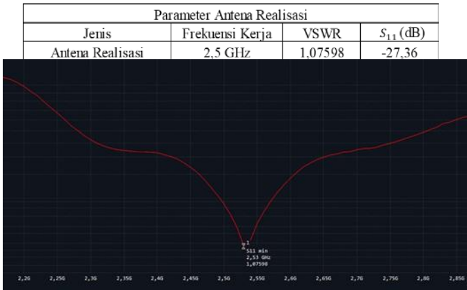
GAMBAR 4.4 VSWR REALISASI
