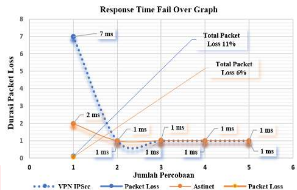
GAMBAR 9. (Response Time Failover).
