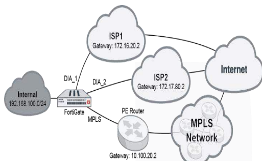
GAMBAR 2. Alur Traffic Steering 2 ISP.
