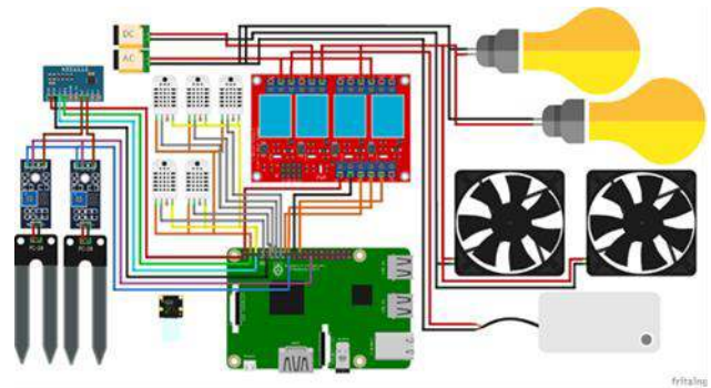
GAMBAR 2 Design Kabel
