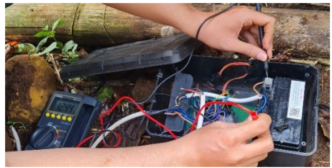
GAMBAR 7. Pengukuran Power Supply
