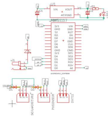
GAMBAR 4 (Wiring Schematic)
