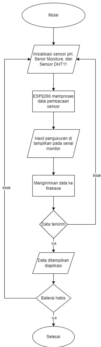
GAMBAR 3 (Flowchart sistem)
