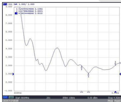
GAMBAR 7. VSWR Perban 3.5GHz
