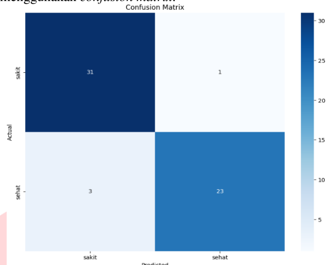
GAMBAR 4. Confusion Matrix
