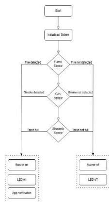
GAMBAR 1 (Flowchart)
