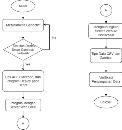
GAMBAR 4 Flowchart Blockchain
