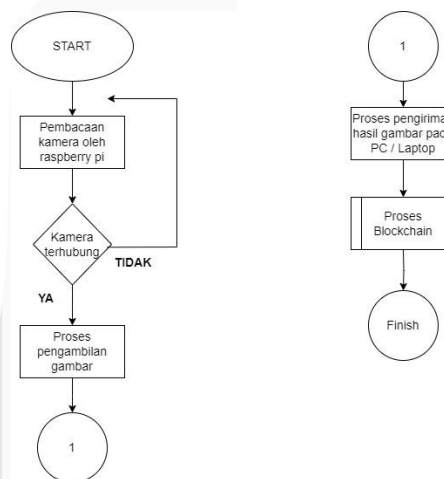
GAMBAR 3 Flowchart Kamera
