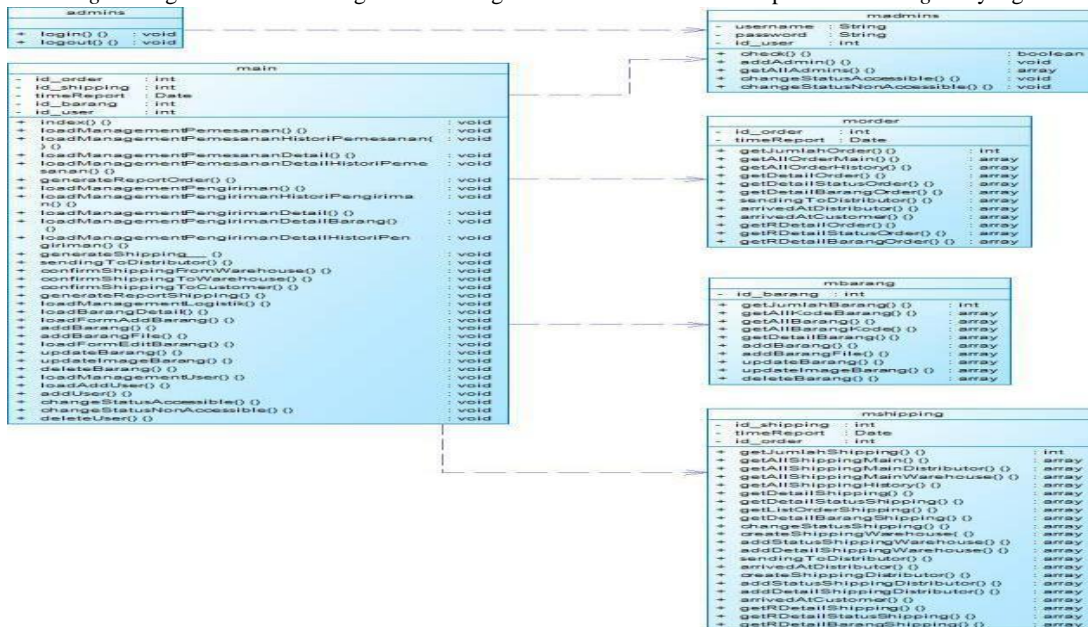
Gambar 6. Class Diagram
