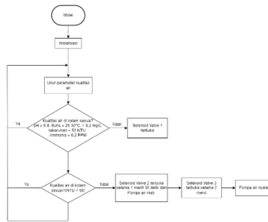
GAMBAR 1. Alur sistem monitoring
