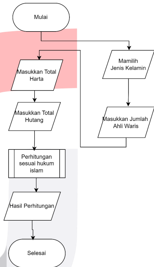
GAMBAR 4. 1. Flowchart Program
