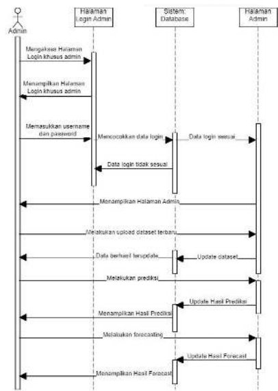
GAMBAR 7 Sequence Diagram Admin
