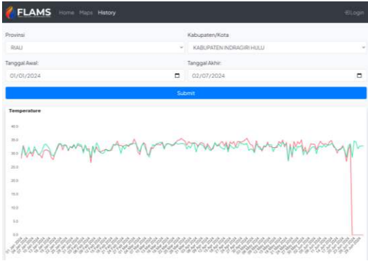
GAMBAR 10 Halaman History
