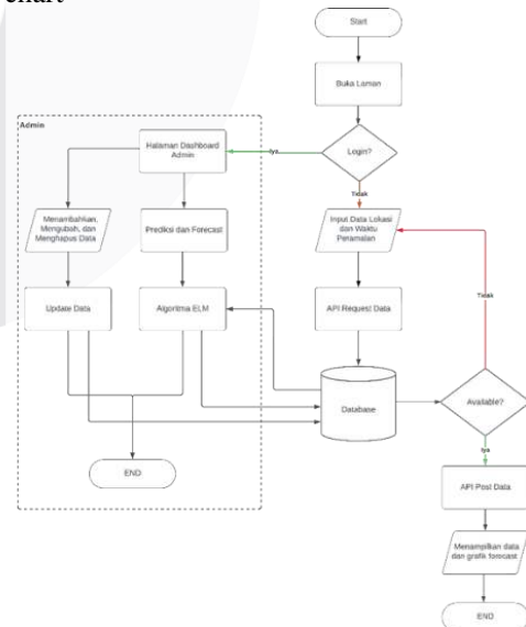
GAMBAR 2 Flowchart
