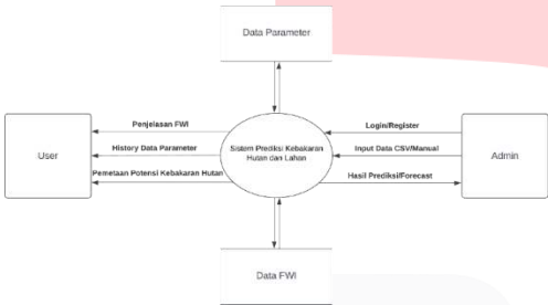
GAMBAR 3 Data Flow Diagram Level 0
