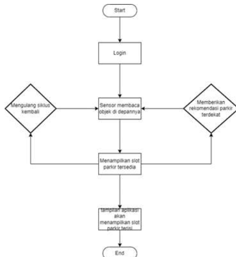
GAMBAR 3. 1 Flowchart
