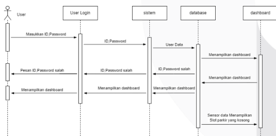
GAMBAR 3. 2 Sequence diagram
